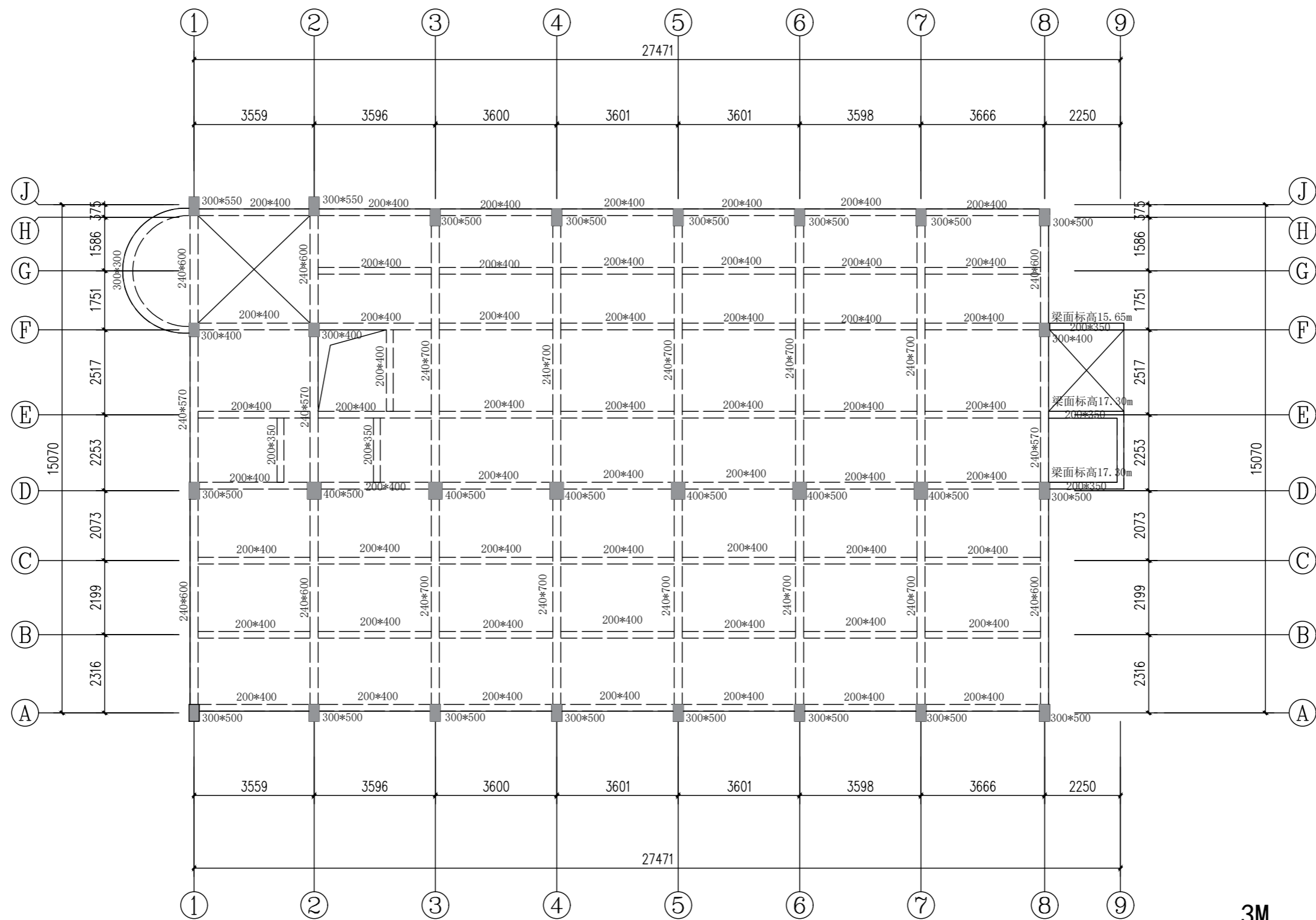
5层 (5层高3.20m, 楼板厚0.10m)
