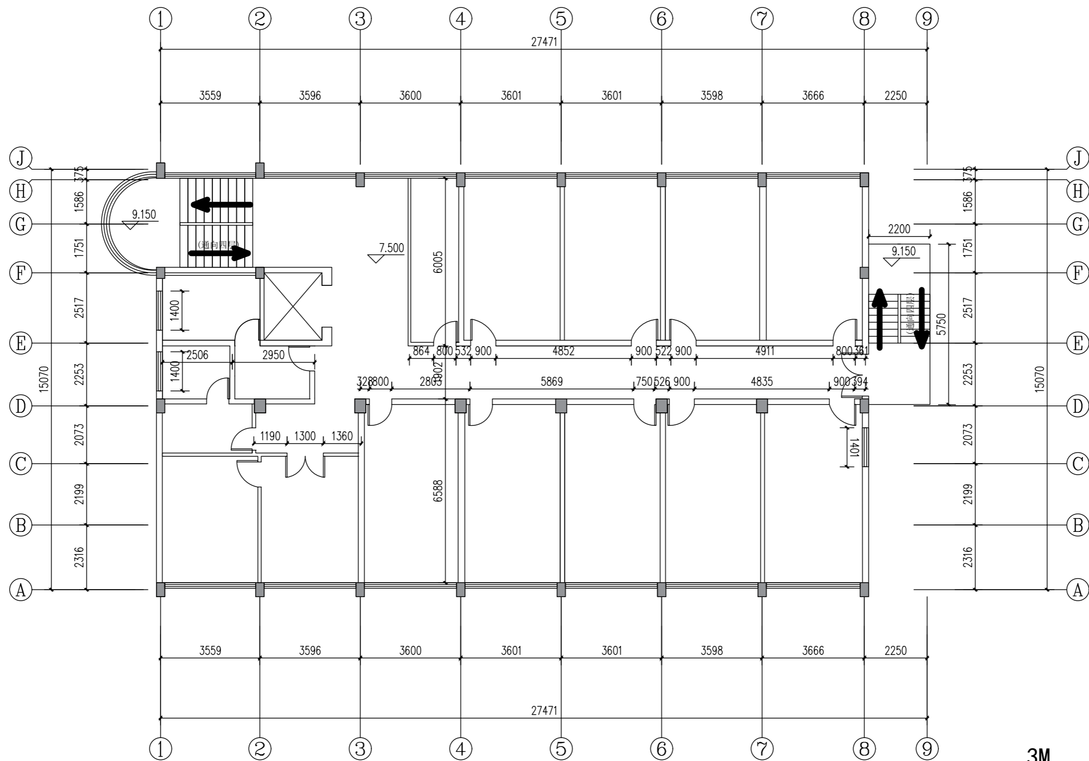
3层 (层高3.20m, 楼板厚0.10m)
