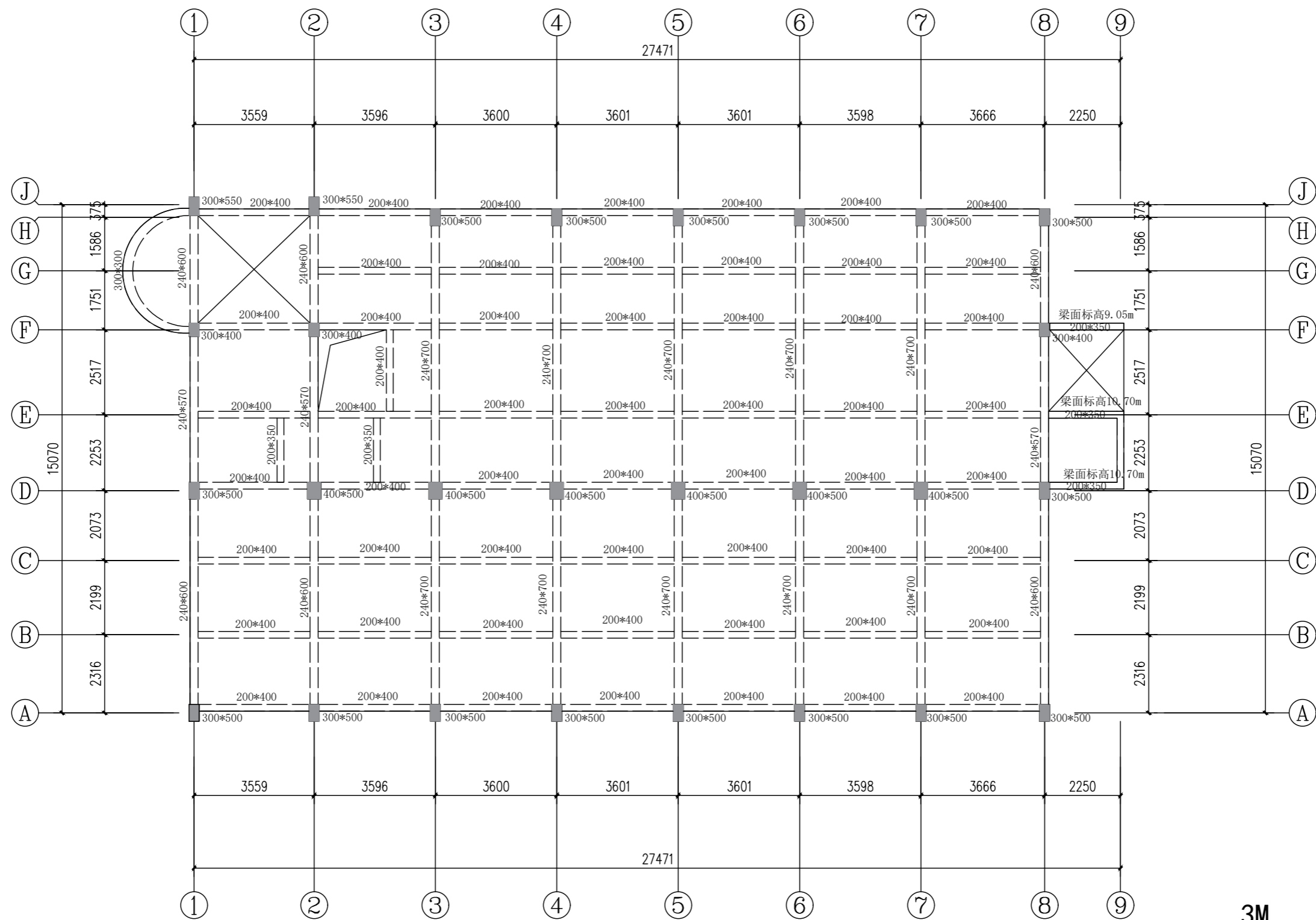
3层 (3层高3.20m, 楼板厚0.10m)
